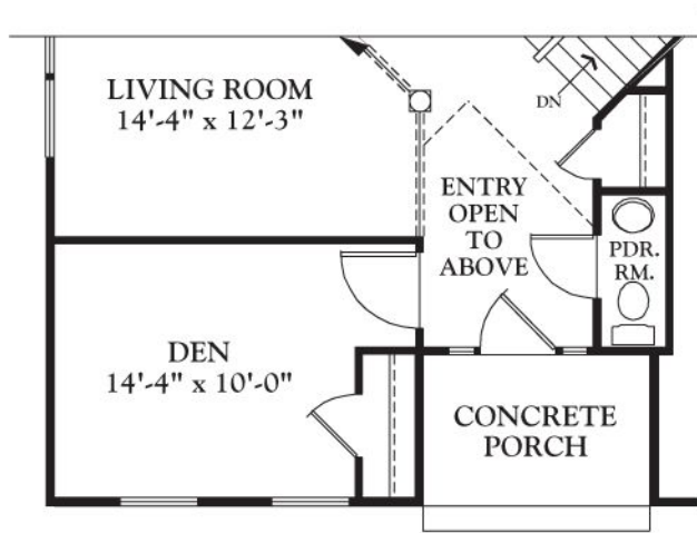
1st Floor With Opt. Den
